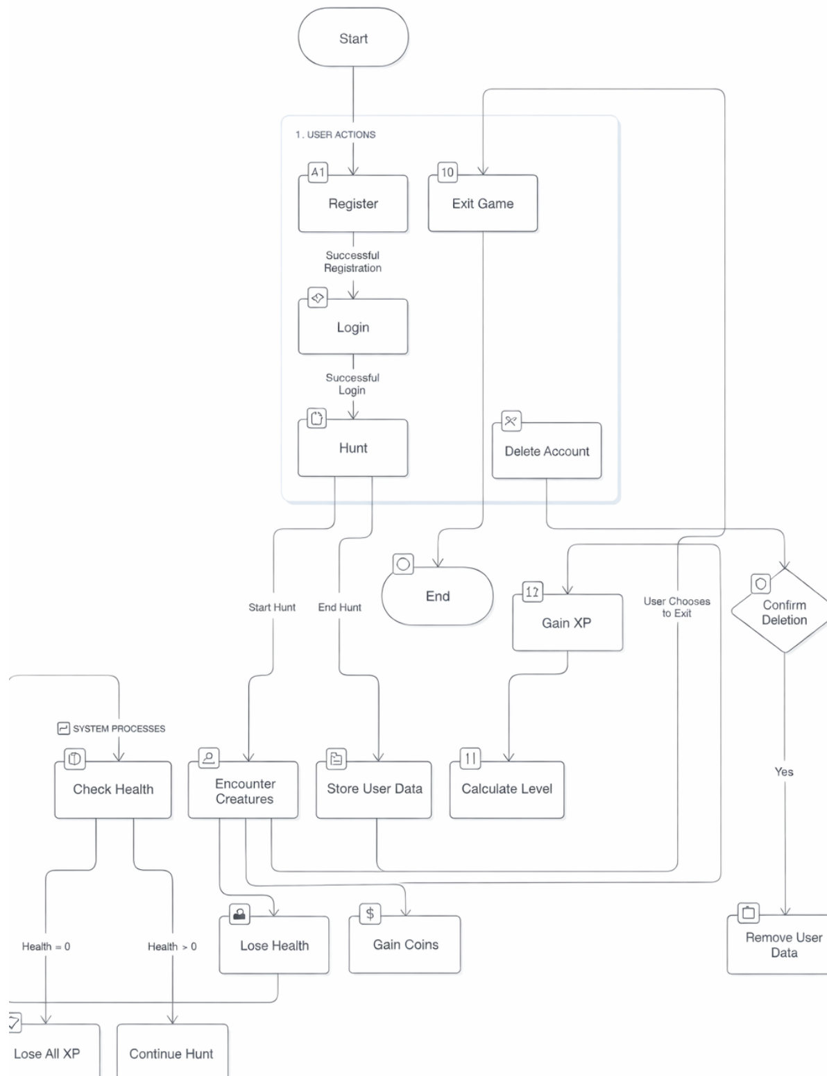
RPG Game System Flowchart
